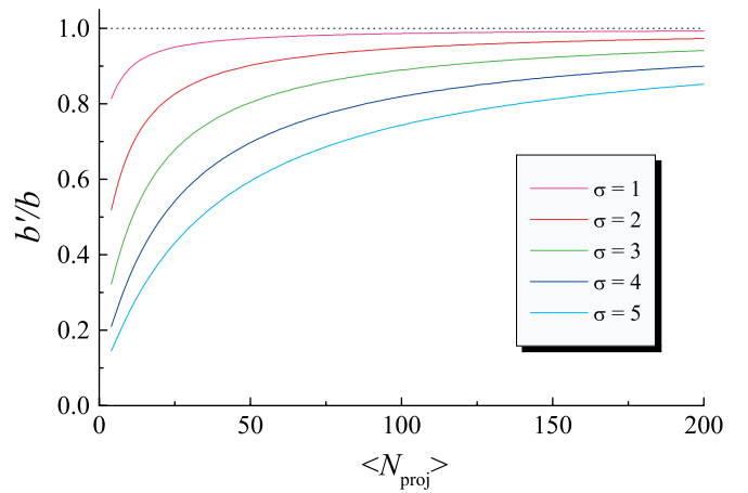
FIG. 1. (Color online) The ratio b'/b as a function of the average number of projectile wounded nucleons \langle N_{\text{proj}} \rangle in Pb-Pb collisions for several values of the dispersion \sigma of N_{\text{proj}} . The uppermost line corresponds to \sigma = 1 , the lower one to \sigma = 2 , etc.
