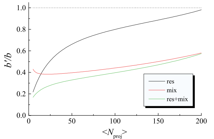
FIG. 2. (Color online) b'/b vs \langle N_{\text{proj}} \rangle in Pb-Pb collisions. The upper curve (“res”) shows the effect of calorimeter resolution; the middle one (“mix”) represents the mixing model; the lower curve (“res+mix”) combines the effect of calorimeter resolution and the mixing-model prediction.
