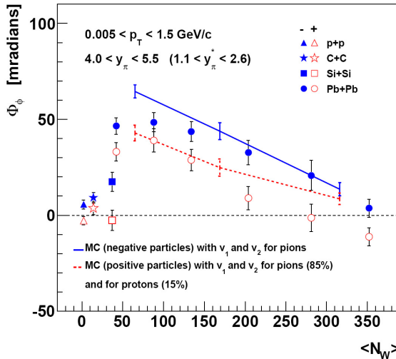
Fig. 3. \Phi_\phi as a function of the number of wounded nucleons for positively and negatively charged particles produced in various colliding systems: p+p , C+C , Si+Si and Pb+Pb at 158A GeV. The solid (dashed) line connects three points which represent the collective flow effect for negative (positive) particles.
