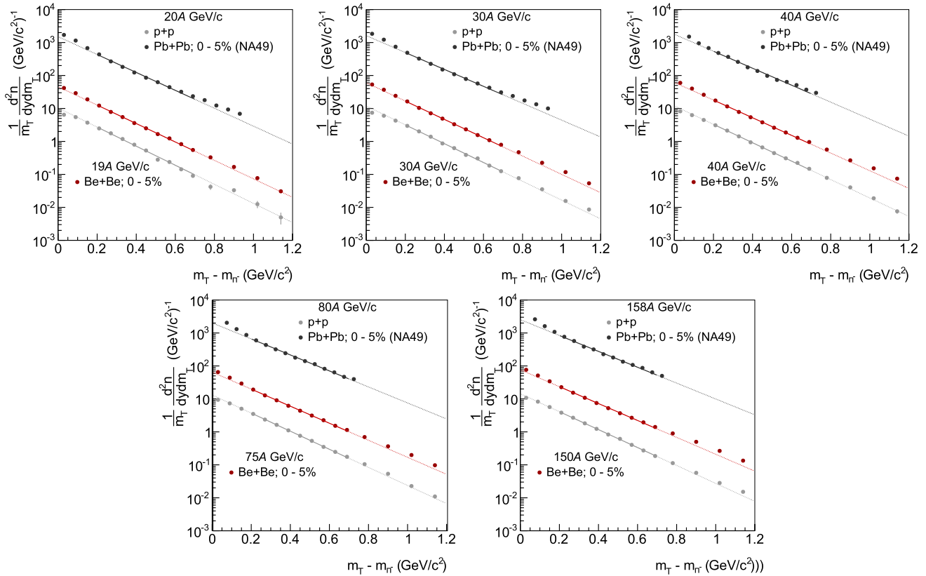
Fig. 13 Transverse mass spectra \frac{1}{m_T - m_\pi} \frac{d^2n}{dy dm_T} of negatively charged pions produced in central Be + Be collisions at the SPS energies. Statis-
