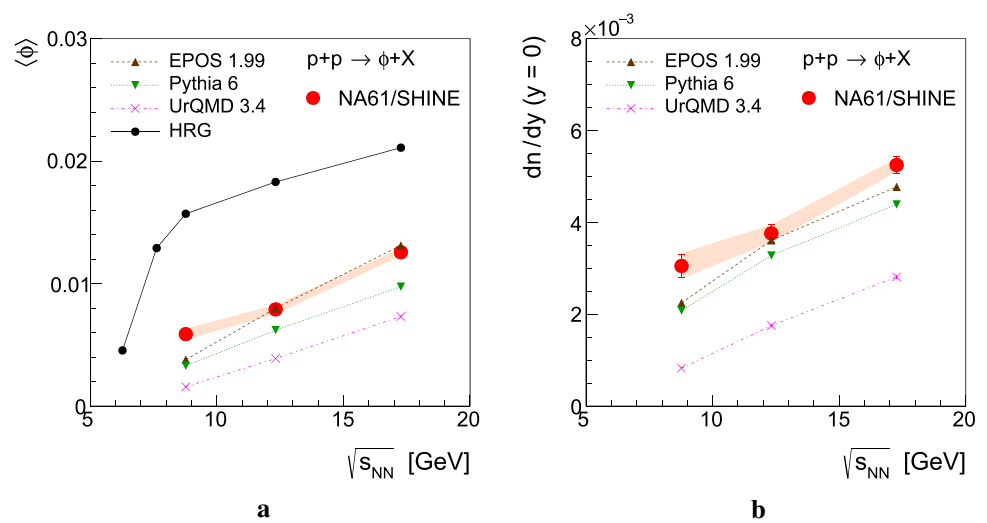
Fig. 17 Energy dependence of a total yields and b midrapidity yields of \phi mesons in p + p collisions at SPS energies. Also shown are the results of microscopic model calculations (EPOS, PYTHIA, UrQMD) as well as the hadron resonance gas model (HRG). Vertical bars show statistical uncertainties, while red bands systematic ones
