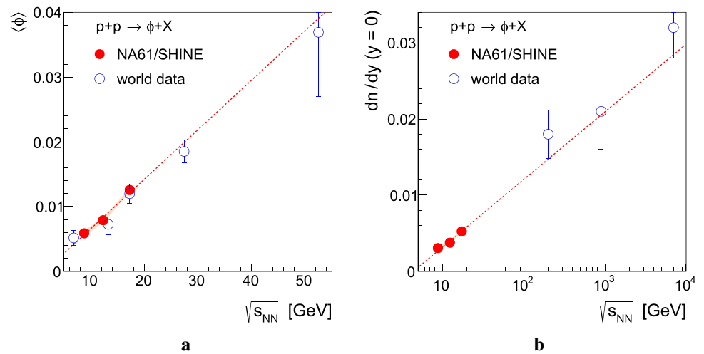
Fig. 16 Energy dependence of a total yields and b midrapidity yields of \phi mesons in p + p collisions. World data on total yields come from Refs. [9–13], while on midrapidity yields come from Refs. [15, 17, 18]. Red dashed lines are fits to guide the eye (see text). Red bands show systematic uncertainties of the NA61/SHINE results, statistical ones are smaller than the markers; for the world data vertical bars are either statistical or total uncertainties depending on what is available (see text)
