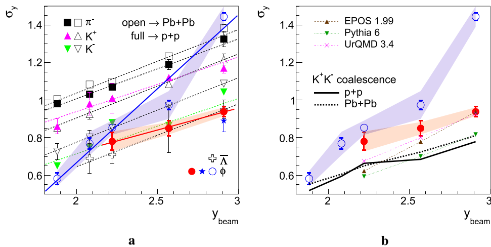
Fig. 18 a Widths of rapidity distributions of various particles in p + p (full symbols) and central Pb + Pb collisions (open symbols) as a function of beam rapidity. Full red circles are results of this analysis, the star is the p + p NA49 measurement [13], other p + p points come from NA61/SHINE [25, 44], while the Pb + Pb points from NA49 [21, 42, 43, 48]. Lines are fitted to points to guide the eye. b Comparison
