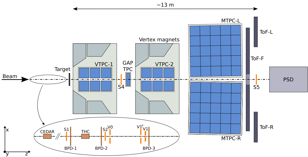
Fig. 1 Schematic layout of the NA61/SHINE detector system (horizontal cut in the beam plane, not to scale). Also outlined are the coordinate system used in the experiment and the beam detector configuration used with secondary proton beams in 2009
