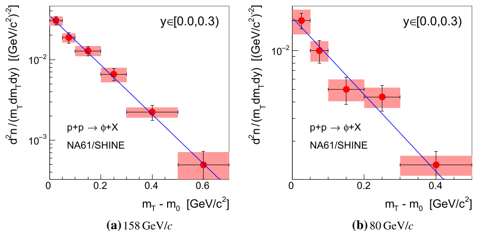
Fig. 12 Transverse mass spectra at midrapidity for 158 GeV/c (left) and 80 GeV/c (right) with statistical (vertical lines) and systematic (red boxes) uncertainties. The horizontal bars indicate bin sizes. The straight lines are the fits of Eq. (10) to the data points
