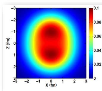
{}^9\text{Be}
